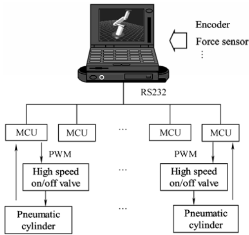
Fig. 9. Distributed control system of the master arm
