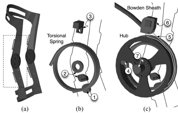
Fig. 1. (a) Structure of the commercial knee brace without padding or straps. The dashed box indicates the close-up view shown in (b) and (c). (b) Close-up of the torsional spring, along with (1) the spring-brace anchor attached to the shank. (2) A Hall-effect goniometer, composed of an annular magnet fixed and centered on the distal lateral hinge and a hall sensor attached to shank, measures brace angle. Part (3) is the Bowden sheath-brace anchor, which is attached at the thigh. The rest of the device is shown in (c), including the hub with a built-in slot (4) for attachment to the spring. The position of the hub is controlled by excursion of Spectra cable (5) wrapped and anchored to it. The cable passes through Bowden sheath attached to the sheath-brace anchor using a custom-made coupler (6). The hub rotates about a steel shaft (not shown) centered at the distal lateral hinge. The angular displacement of the hub relative to the shaft is measured by an encoder (7) coupled with the hub using a spring-suspension platform. This platform keeps the encoder fixed to the shaft while the spring deformation creates an increase in height (direction along rotation axis) of the hub. Torque exerted by the device is determined by using the difference between the angle measured by the encoder and that of the Hall-effect goniometer.
