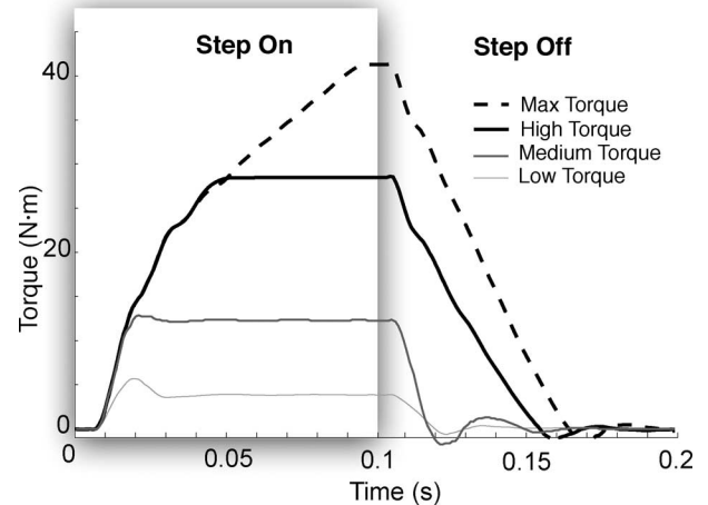
Fig. 3. Step responses (each curve is the average of three trials) for low, medium, and high torques. In this experiment, we measured torque by the deflection in the spring.
