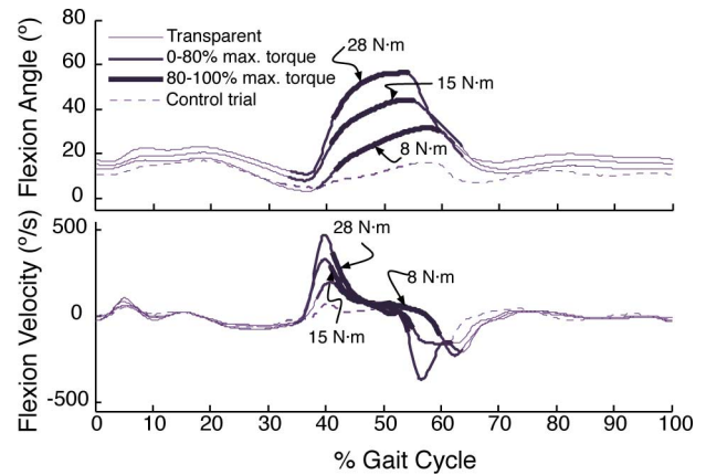
Fig. 8. In subject S5, knee flexion angle and velocity increase during the assistance, but the kinematics return to their typical values once the assistance stops.
