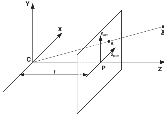
Fig. 9. Perspective projection
