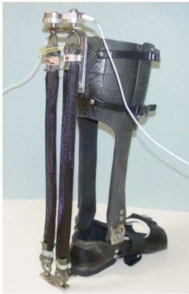
Figure 1 Subjects wore a custom fit orthosis on their left lower limb. The orthosis was hinged at the ankle to allow free sagittal plane rotation. Soleus EMG activation was recorded and processed to be used to control air pressure in the artificial pneumatic muscles proportionally. As air pressure increased, the artificial muscles started to develop tension and become shortened, allowing the powered exoskeleton to provide plantar flexor torque controlled by soleus muscle activation.
