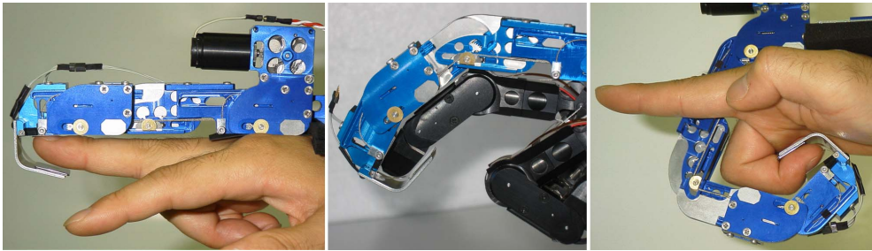
Fig. 26 Master finger mechanism (MAF) following various finger flexions.
