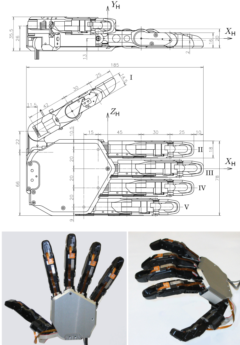
Fig. 13 Overall profile of the latest model.
