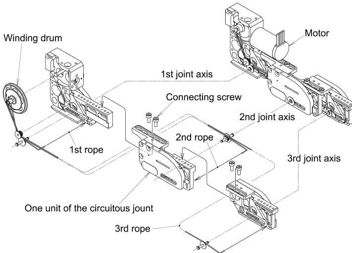
Fig. 27 Adjustable tandem connection of three joint units.
