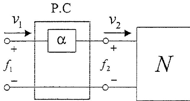
(a) Series or velocity conserving Passivity Controller.
