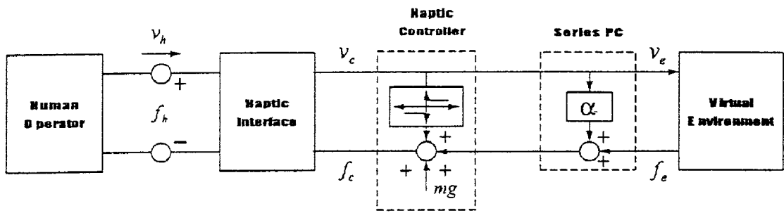
Fig. 11 15 "Excalibur" 3-axis, high force output, haptic interface system
