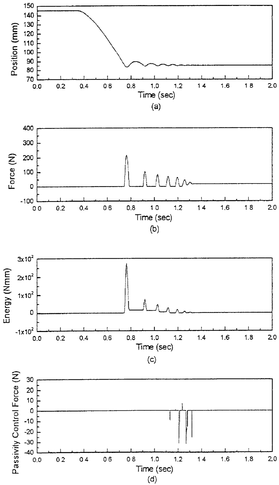
17 Fig. 13 Contact with high stiffness with PC.
