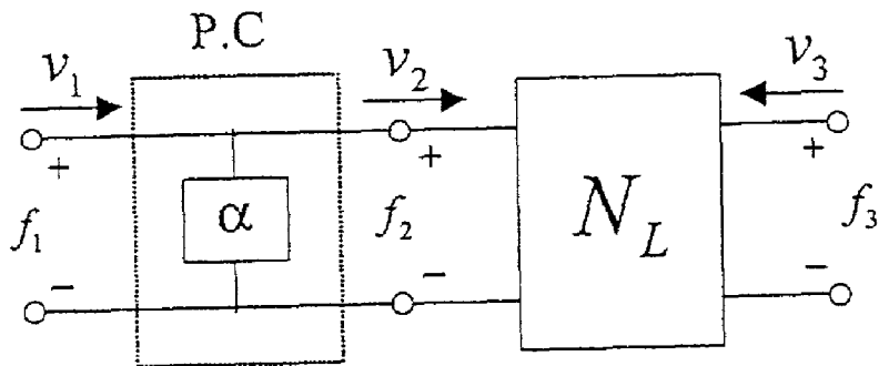
(b) Parallel or force conserving
