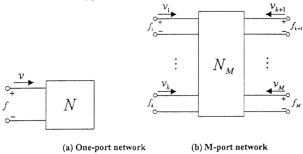
5 Fig. 1 One-port and M-port networks
