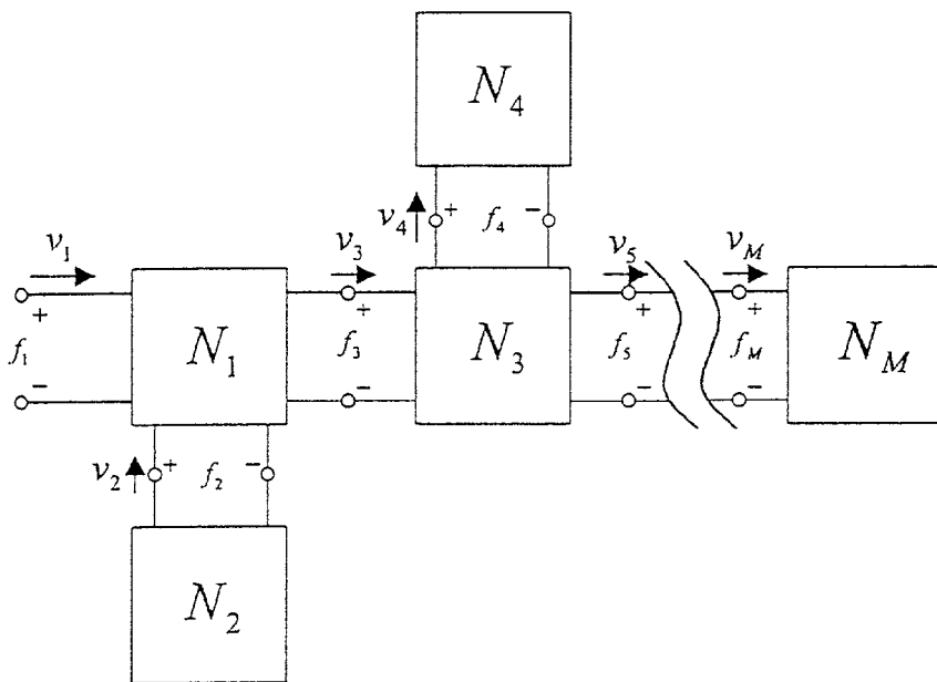
6 Fig. 2 Example of arbitrarily connected network system with one open-end.
