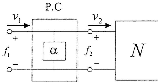
(b) Parallel or force conserving Passivity Controller.
