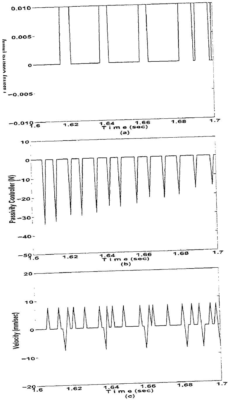
Figure 11: Trajectories Zoomed in t = 1.6\text{sec} to 1.7\text{sec} to show the noise effect at low velocity
