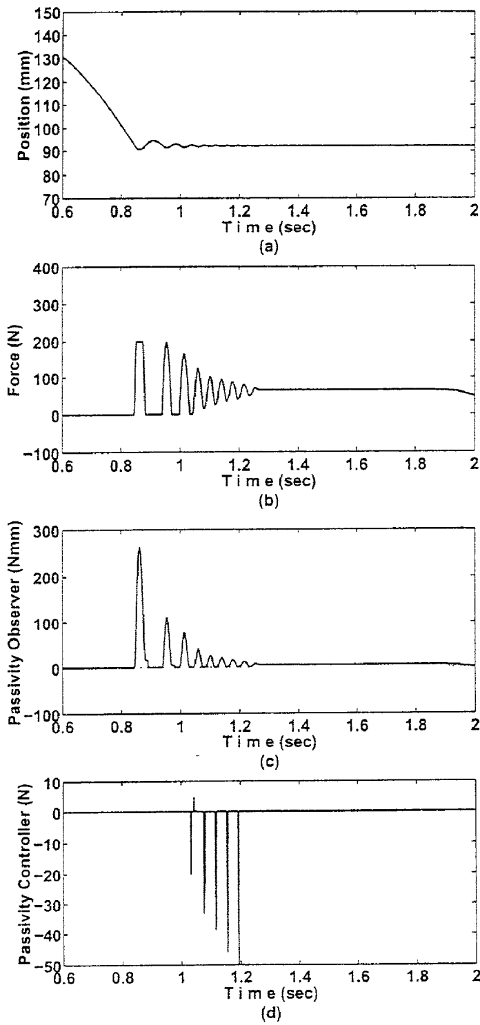
22 Figure 12: Contact with high stiffness with both PC and resetting
