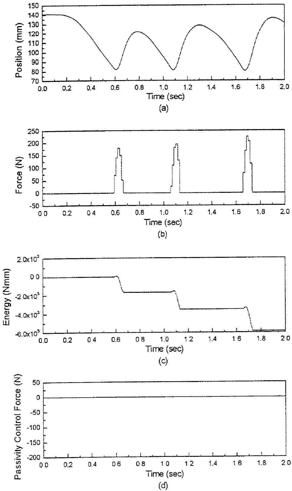
Fig. 45 Delayed environment without PC.
