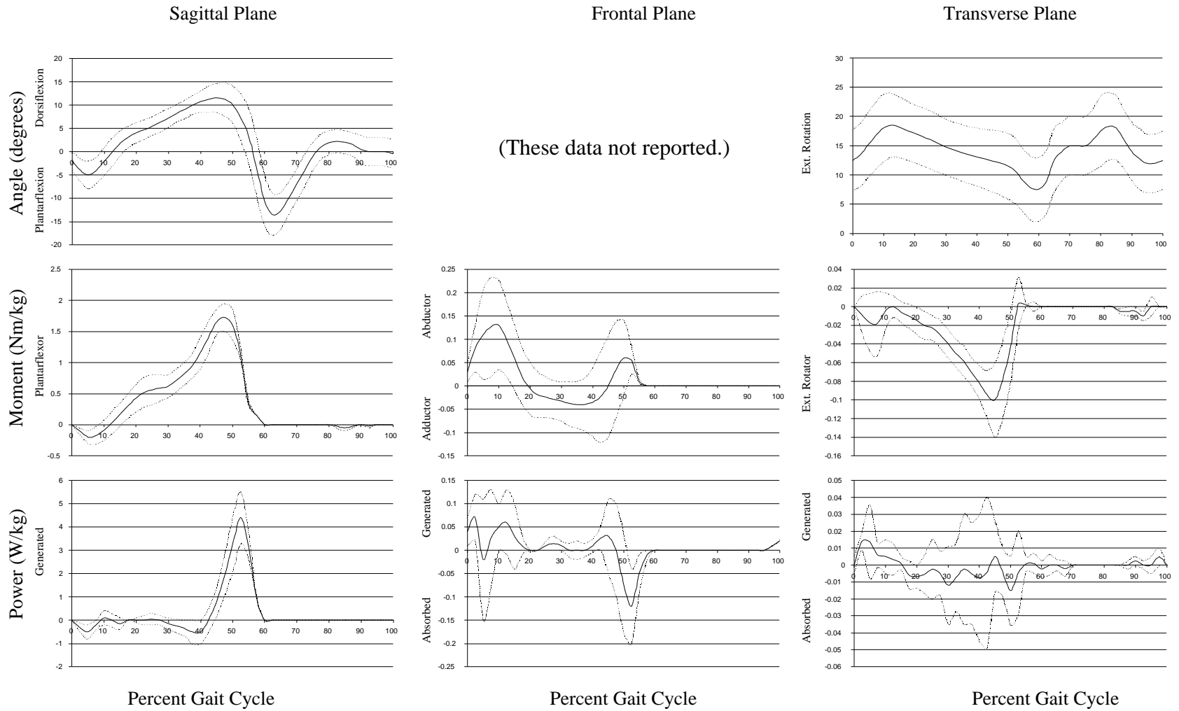
Figure A-3. Ankle joint angles, moments, and powers in the sagittal, frontal and transverse planes during one cycle of normal walking.
