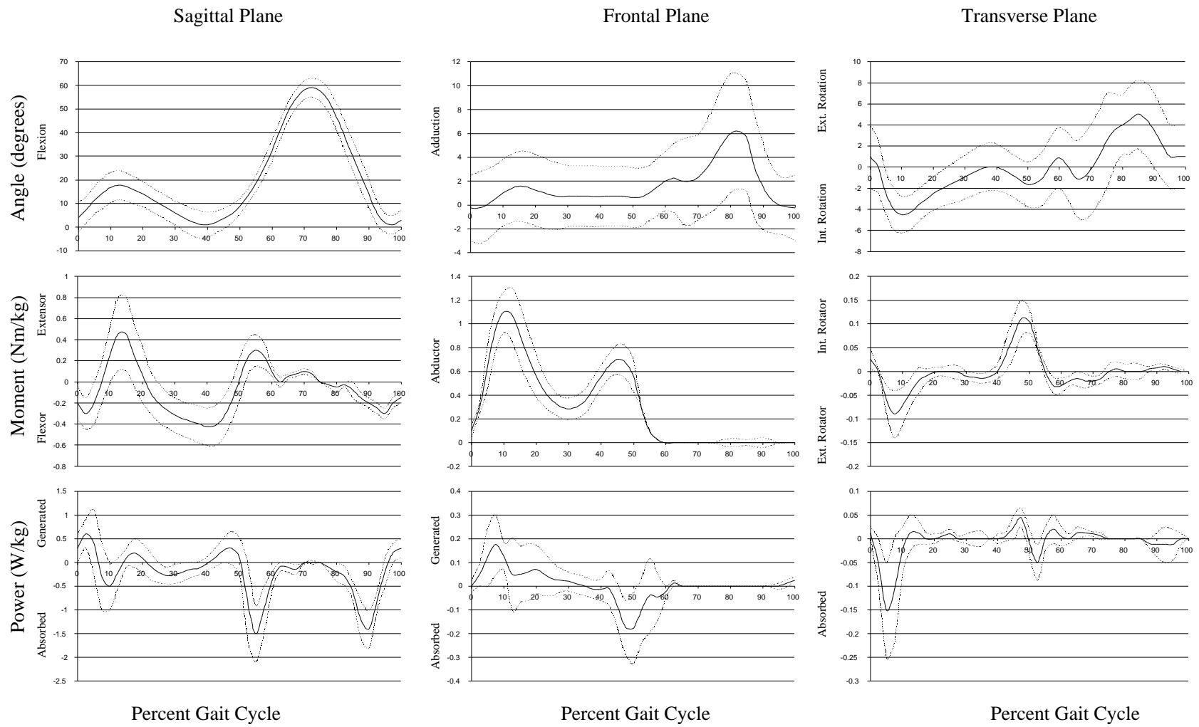
Figure A-2. Knee Joint angles, moments, and powers in the sagittal, frontal and transverse planes during one cycle of normal walking.
