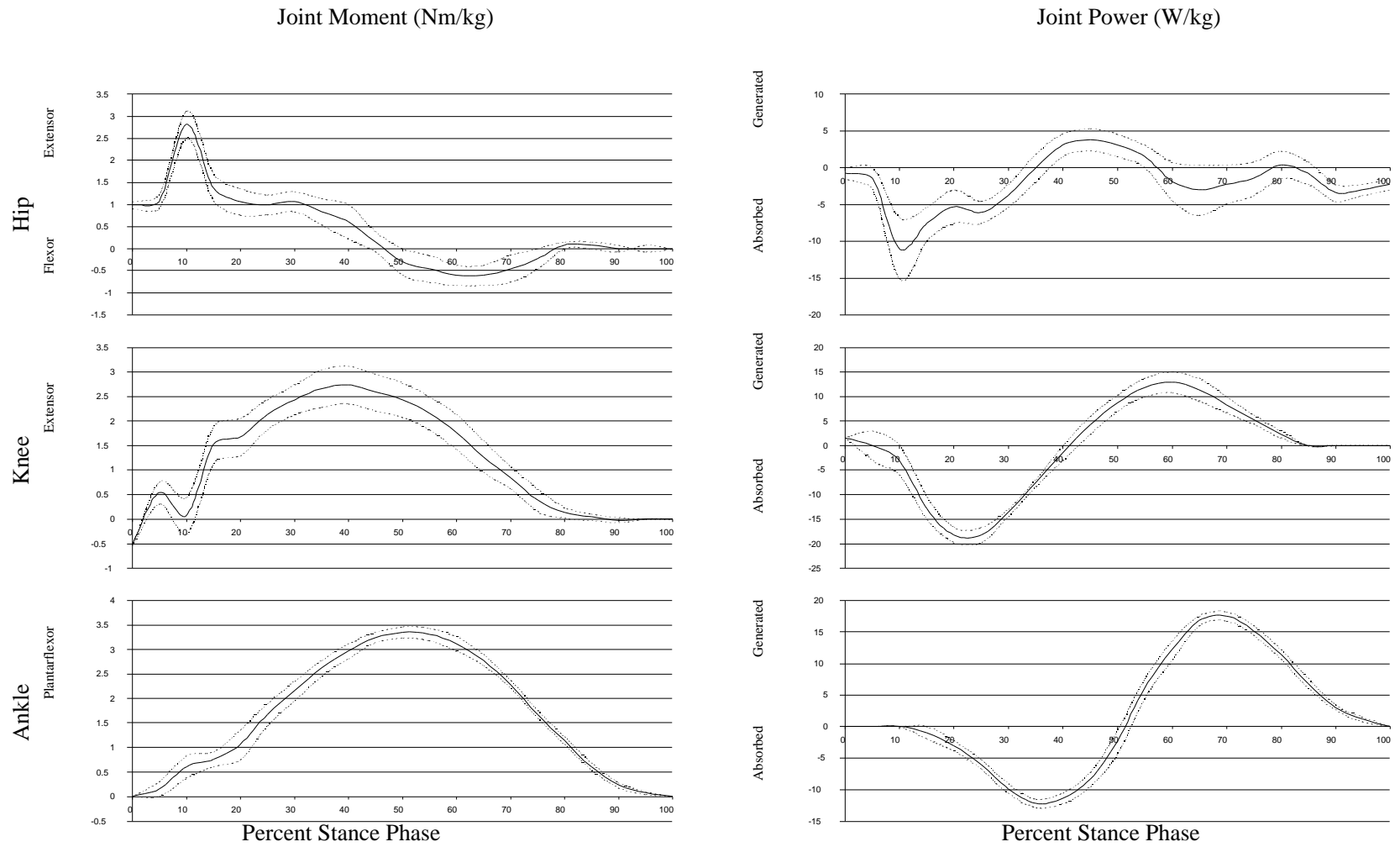
Figure A-6. Sagittal plane joint moments and powers during the stance phase of running at a moderate pace (3.8 m/s). (Solid lines are mean values and dotted lines are \pm one standard deviation.)
