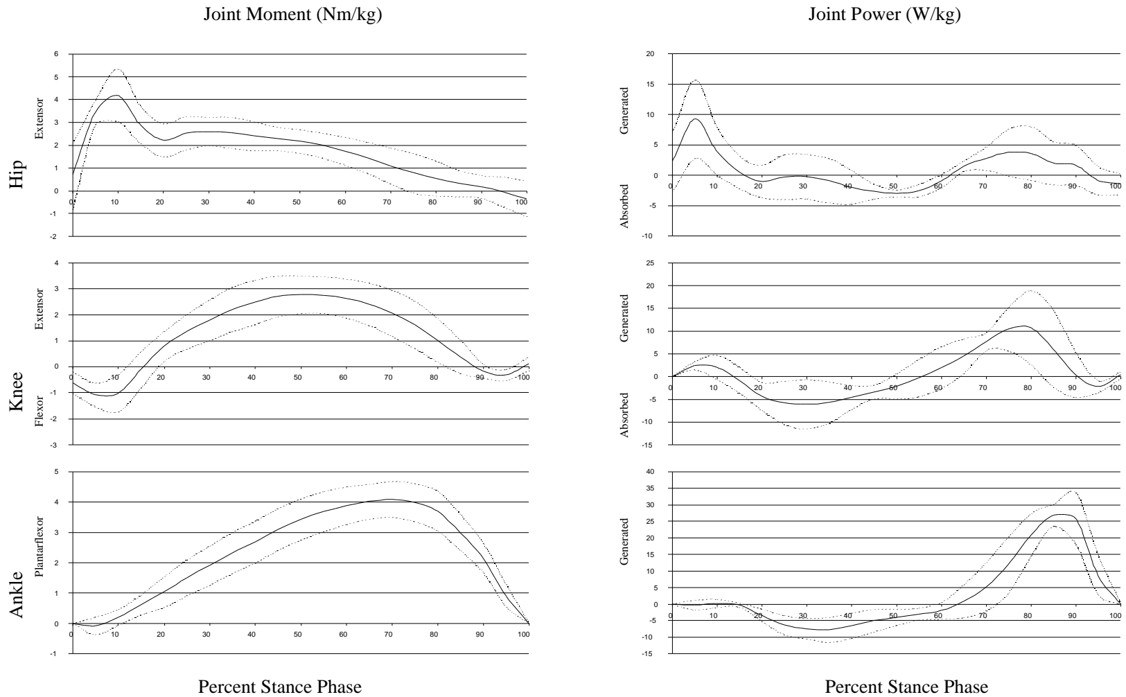
Figure A-10. Sagittal plane joint moments and power during the stance phase before toe-off of a running vertical jump. (Solid lines are mean values, and dotted lines are \pm one standard deviation.)
