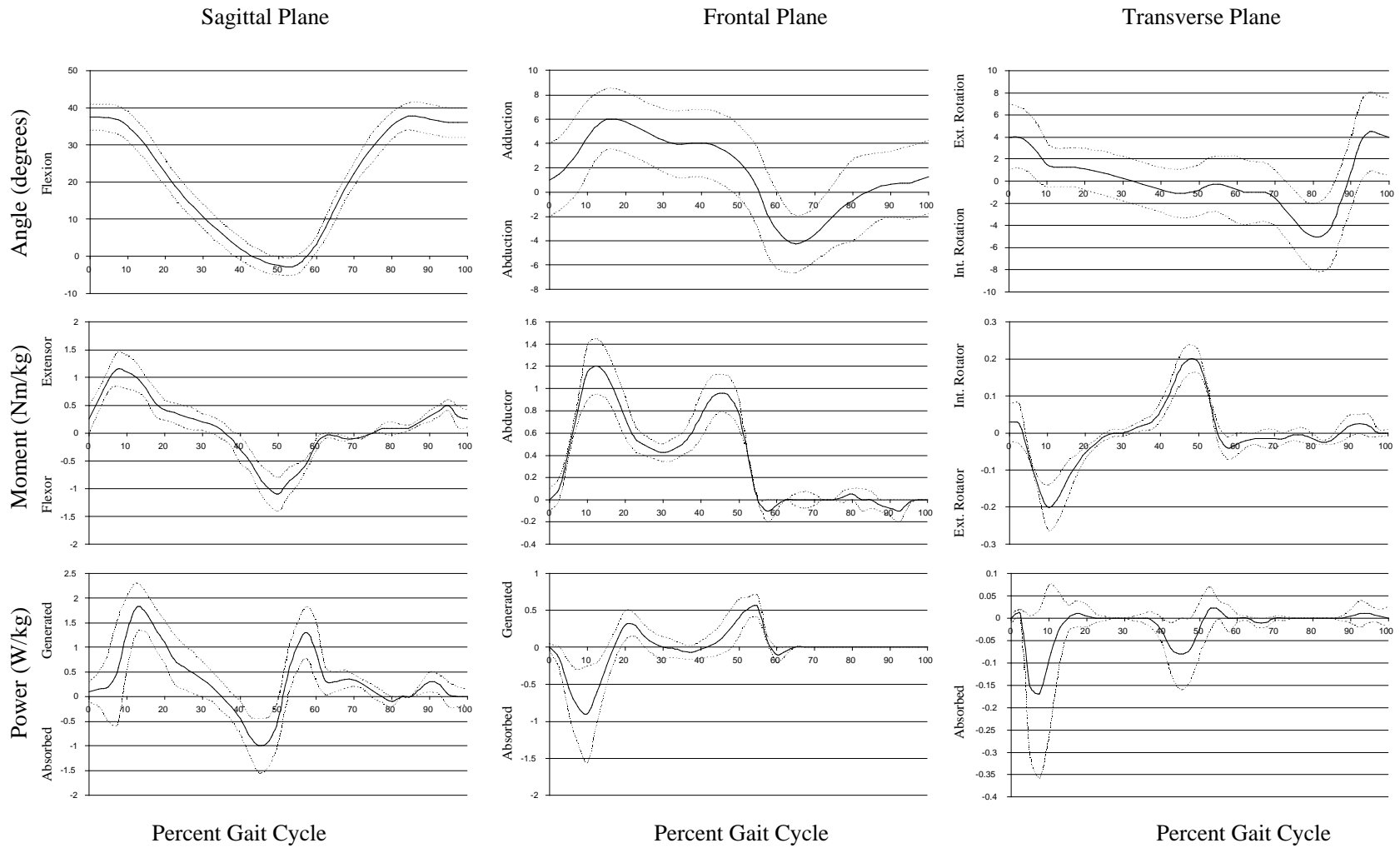
Figure A-1. Hip joint angles, moments, and powers in the sagittal, frontal, and transverse planes during one cycle of normal walking. (Solid lines are mean values and dotted lines are \pm one standard deviation.)
