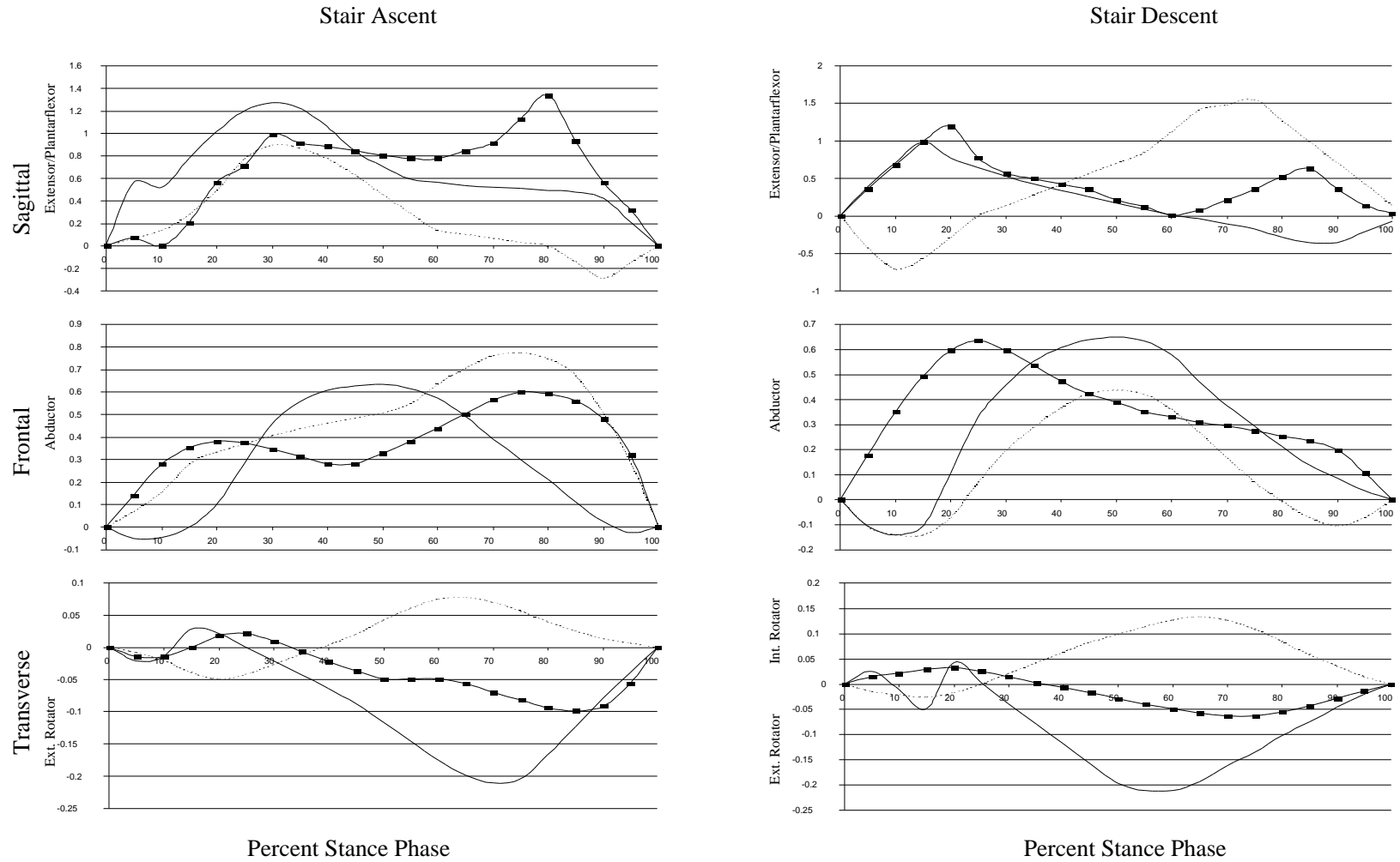
Figure A-8. Joint moments in the sagittal, frontal, and transverse planes during stance phase of stair ascent and descent. (— = hip, ---- = knee, —■— = ankle). (Values are in newton meters per kilogram.)
