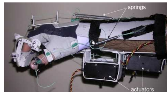
Fig. 2. Overview of the complete rehabilitation system.
