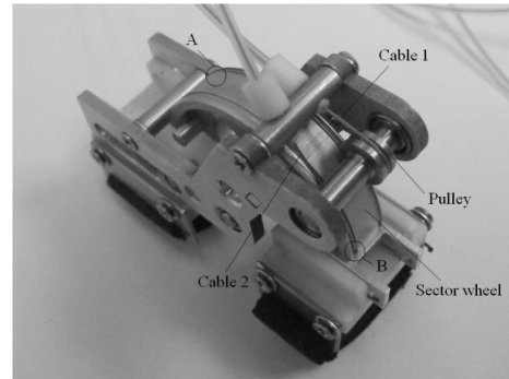
Fig. 4. Detail of Prototype of PIP module
